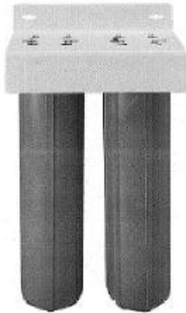
MODEL: TGST-1.5
